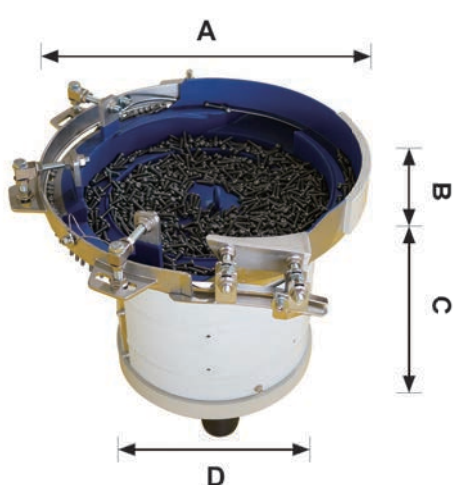
螺絲震動送料機 Screw Vibration Feeder
