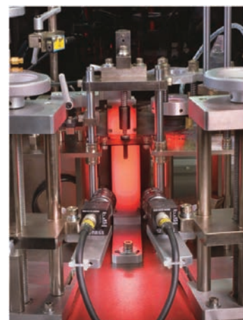
針孔檢測機構 Pinhole Inspection mechanism
