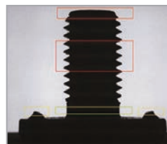
焊點高度/桿徑/螺牙 welding points / shank OD / thread / pitch
